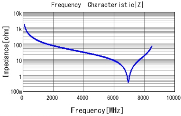
■ GQM22M5C2H1R0CB01 |Z| DC0V, 25degC
