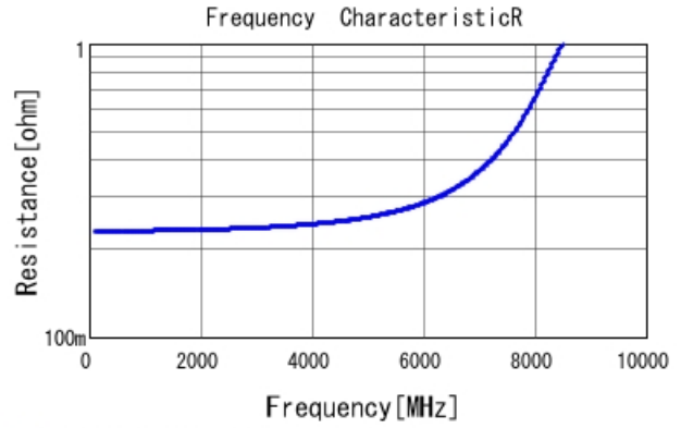
■ GQM22M5C2H1R0CB01 R DC0V, 25degC
