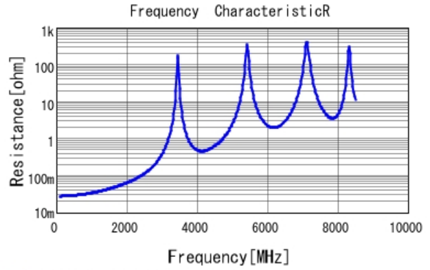
■ GQM22M5C2H200JB01 R DC0V, 25degC
