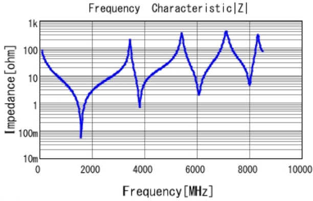
■ GQM22M5C2H200JB01 |Z| DC0V, 25degC
