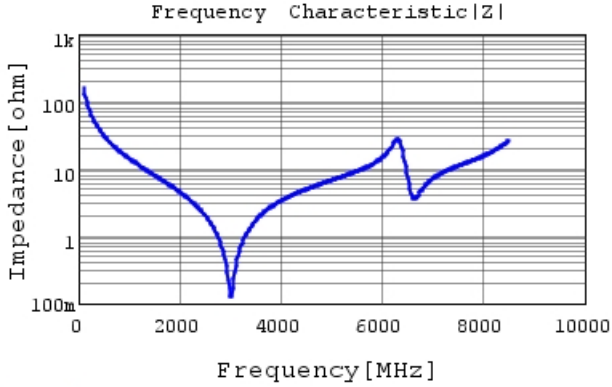
GQM1555C2D100GB01 |Z| DC0V, 25degC
