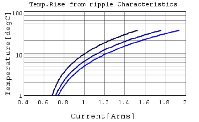
GQM1555C2D100GB01 Temp.rise — 700MHz —
