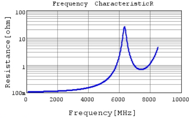
GQM1555C2D100GB01 R DC0V, 25degC
