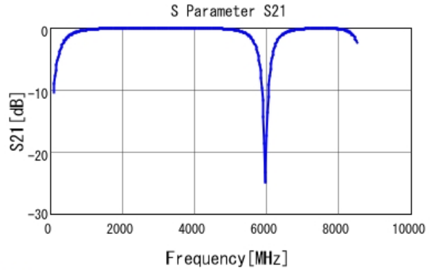
■ GQM22M5C2H5R0BB01 S21 DCOV, 25degC
