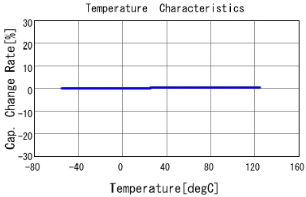
■ GQM22M5C2H5R0BB01 C-Temp. capchange, DCOV, AC1Vrms
