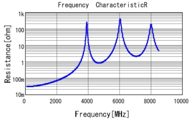
■ GQM22M5C2H150JB01 R DC0V, 25degC
