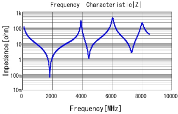
■ GQM22M5C2H150JB01 |Z| DC0V, 25degC
