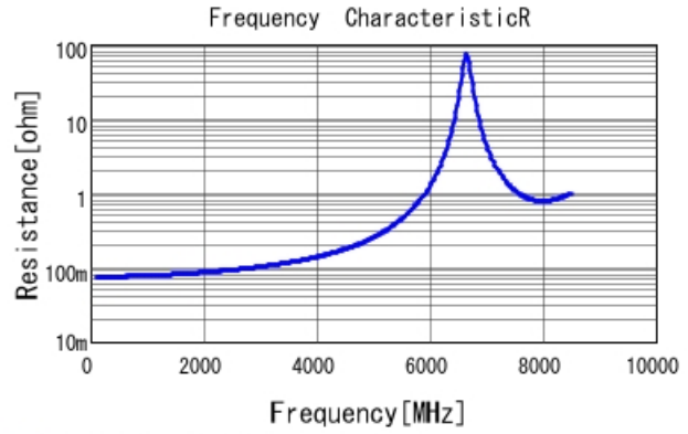
■ GQM1875C2E7R5CB12 R DC0V, 25degC
