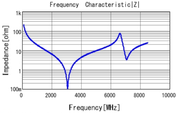
■ GQM1875C2E7R5CB12 |Z| DC0V, 25degC
