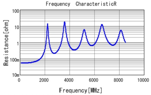
■ GQM1875C2E680JB12 R DCOV, 25degC
