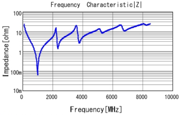
■ GQM1875C2E680JB12 |Z| DCOV, 25degC
