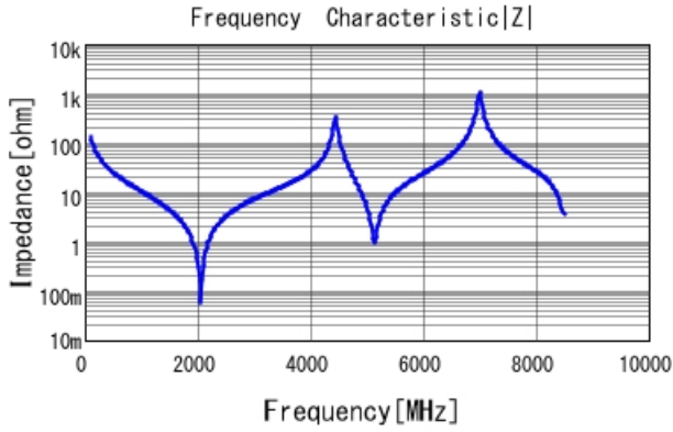
■ GQM22M5C2H120JB01 |Z| DC0V, 25degC
