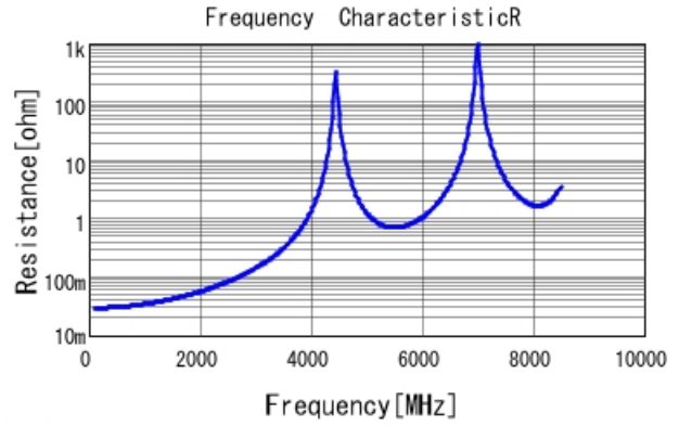
■ GQM22M5C2H120JB01 R DC0V, 25degC
