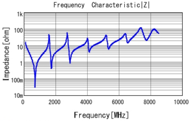
■ GQM22M5C2H101JB01 |Z| DC0V, 25degC
