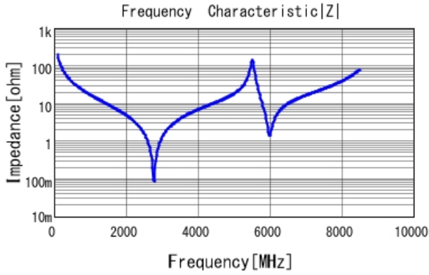
■ GQM2195C2E8R2CB12 |Z| DCOV, 25degC
