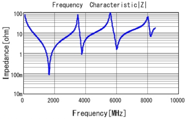
■ GQM2195C2E220JB12 |Z| DC0V, 25degC
