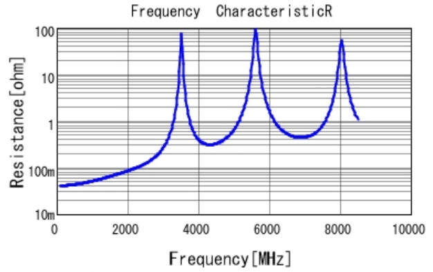
■ GQM2195C2E220JB12 R DC0V, 25degC
