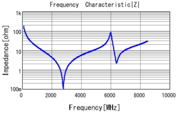
■ GQM1875C2E9R1CB12 |Z| DCOV, 25degC
