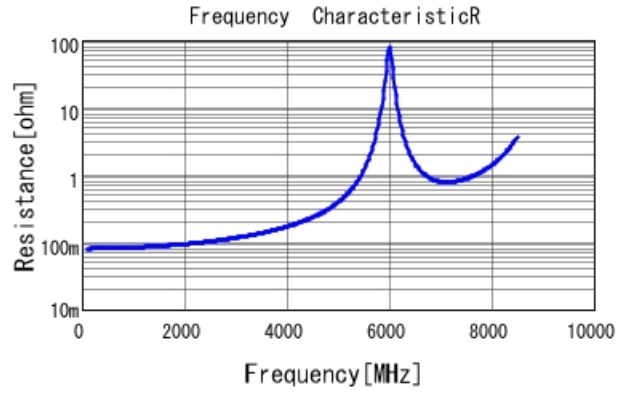
■ GQM1875C2E9R1CB12 R DCOV, 25degC
