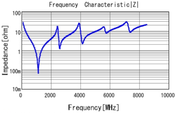
■ GQM1875C2E560JB12 |Z| DCOV, 25degC
