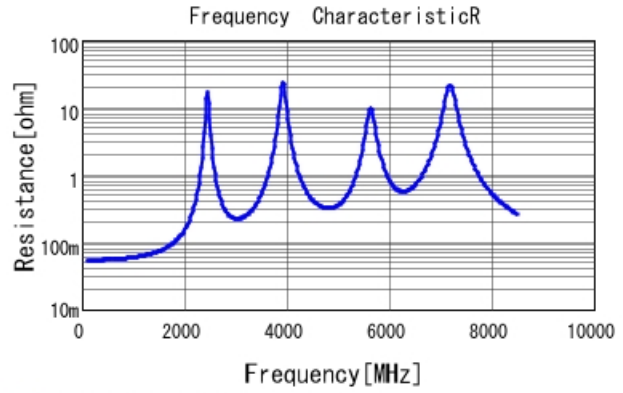
■ GQM1875C2E560JB12 R DCOV, 25degC
