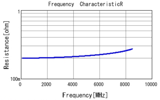
■ GQM2195C2E1R0BB12 R DCOV, 25degC
