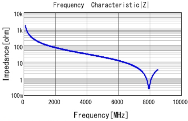
■ GQM2195C2E1R0BB12 |Z| DCOV, 25degC
