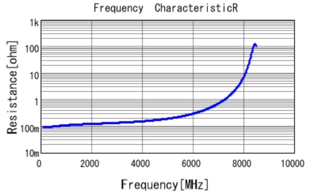
■ GQM1875C2E4R3BB12 R DCOV, 25degC
