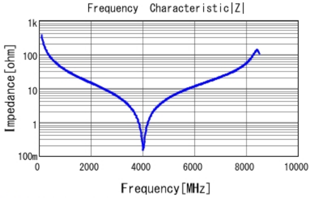
■ GQM1875C2E4R3BB12 |Z| DCOV, 25degC
