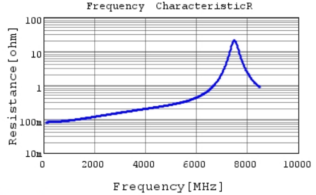
GJM1555C1H9R0WB01 R DCOV, 25degC
