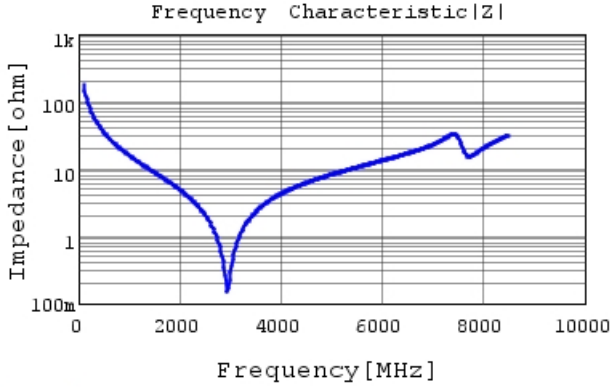
GJM1555C1H9R0WB01 |Z| DCOV, 25degC
