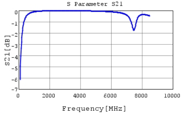
GJM1555C1H9R0WB01 S21 DCOV, 25degC
