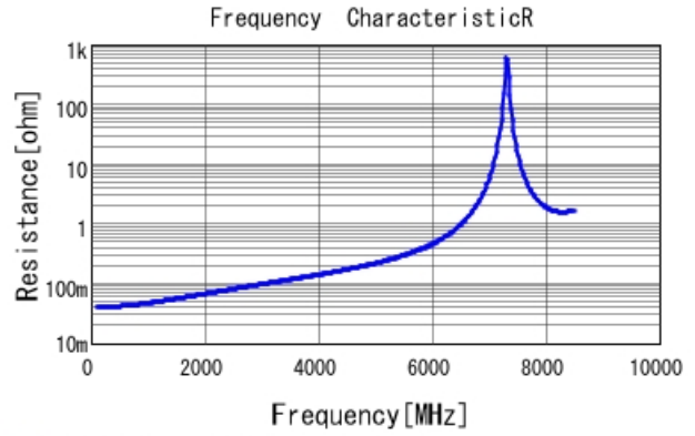
■ GQM2195C2E4R7BB12 R DC0V, 25degC
