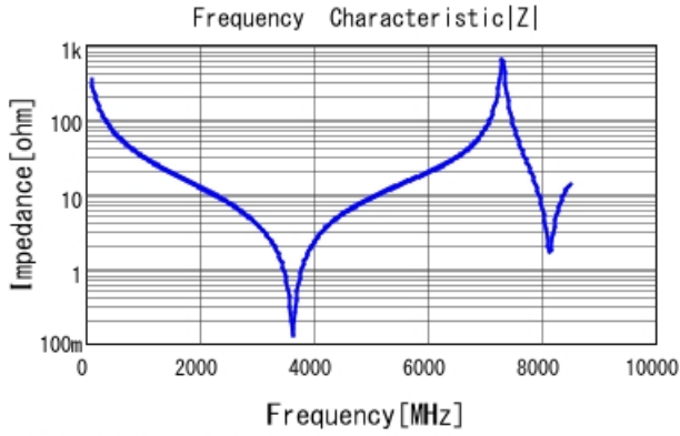
■ GQM2195C2E4R7BB12 |Z| DC0V, 25degC
