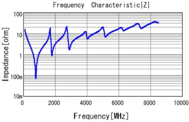
■ GQM2195C2E101JB12 |Z| DC0V, 25degC
