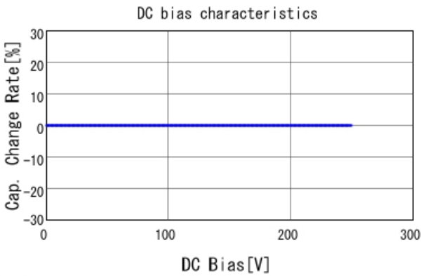
■ GQM2195C2E101JB12 C-DC bias capchange, 25.0degC, AC1V
