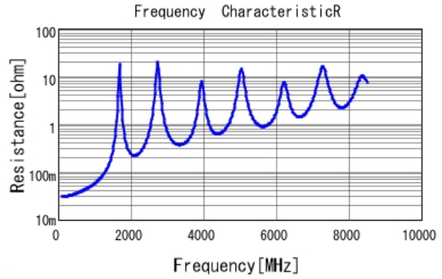
■ GQM2195C2E101JB12 R DC0V, 25degC
