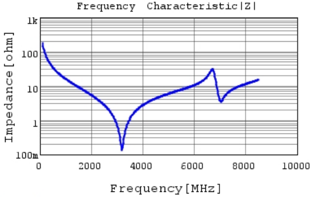
GQM1555C2D9R0BB01 |Z| DC0V, 25degC
