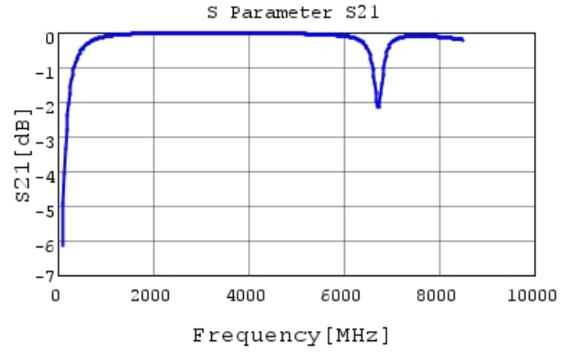
GQM1555C2D9R0BB01 S21 DCOV, 25degC
