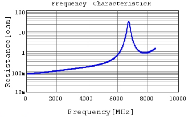
GQM1555C2D9R0BB01 R DC0V, 25degC
