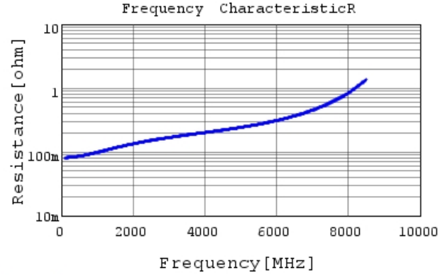
GJM1555C1H7R0WB01 R DC0V, 25degC
