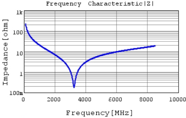
GJM1555C1H7R0WB01 |Z| DC0V, 25degC
