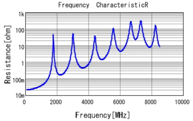
■ GQM22M5C2H820GB01 R DC0V, 25degC
