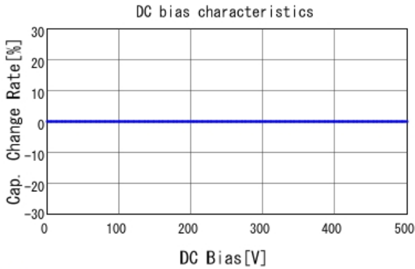
■ GQM22M5C2H820GB01 C-DC bias capchange, 25.0degC, AC1V
