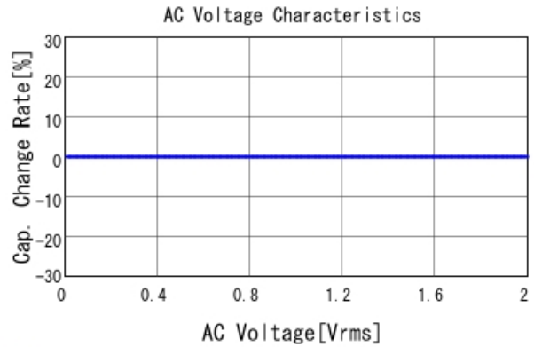
■ GQM22M5C2H820GB01 C-AC Voltage capchange, DC0V, 25.0d
