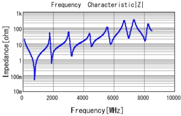
■ GQM22M5C2H820GB01 |Z| DC0V, 25degC
