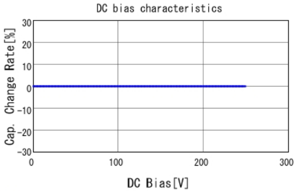
■ GQM1875C2E1R8BB12 C-DC bias capchange, 25.0degC, AC1V
