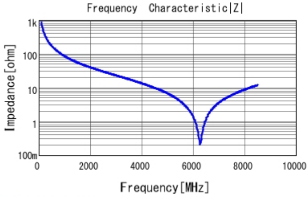
■ GQM1875C2E1R8BB12 |Z| DCOV, 25degC
