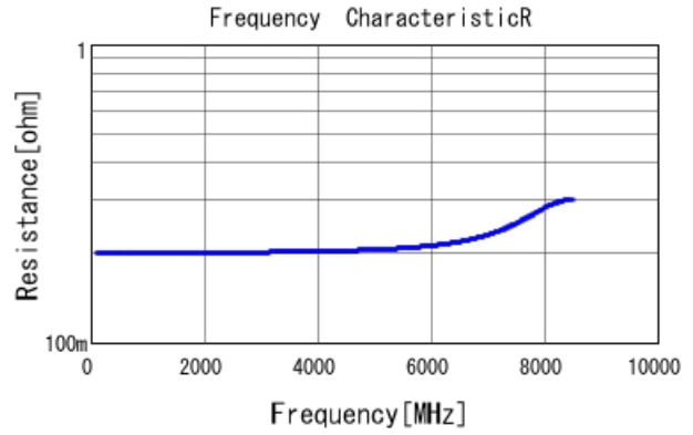
■ GQM1875C2E1R8BB12 R DCOV, 25degC
