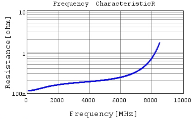
GQM1555C2D3R3BB01 R DC0V, 25degC
