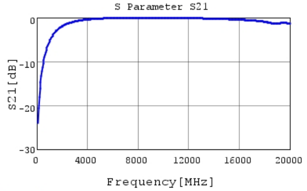
GQM1555C2D1R0BB01 S21 DCOV, 25degC
