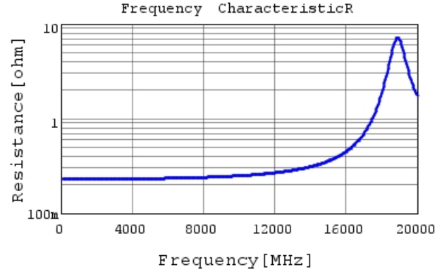
GQM1555C2D1R0BB01 R DC0V, 25degC
