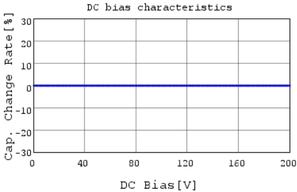
GQM1555C2D1R0BB01 C-DC bias capchange, 25.0c
