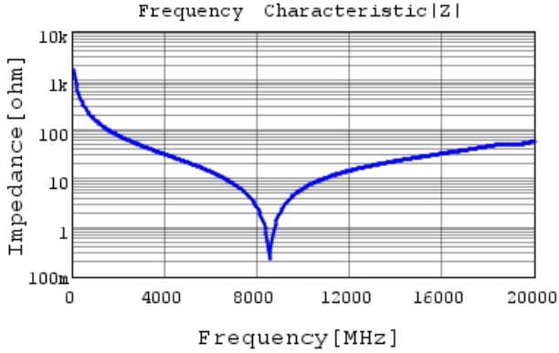
GQM1555C2D1R0BB01 |Z| DC0V, 25degC
