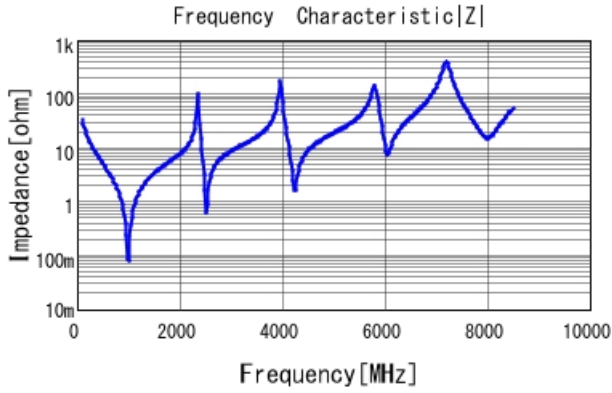
■ GQM22M5C2H470GB01 |Z| DC0V, 25degC
