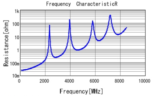
■ GQM22M5C2H470GB01 R DC0V, 25degC
