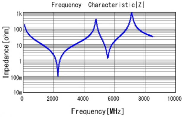
■ GQM22M5C2H100JB01 |Z| DC0V, 25degC
