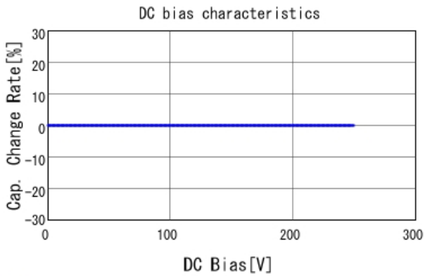
■ GQM2195C2E1R8BB12 C-DC bias capchange, 25.0degC, AC1V
