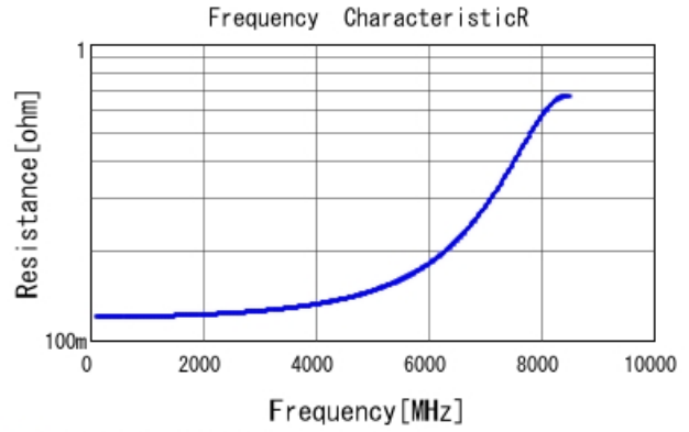
■ GQM2195C2E1R8BB12 R DCOV, 25degC
