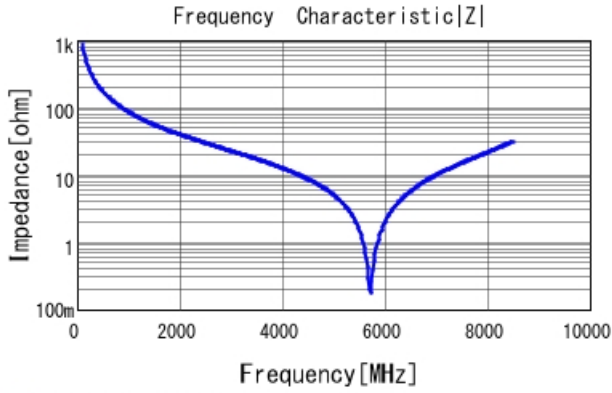
■ GQM2195C2E1R8BB12 |Z| DCOV, 25degC
