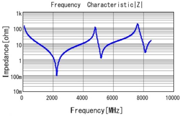
■ GQM2195C2E120JB12 |Z| DC0V, 25degC
