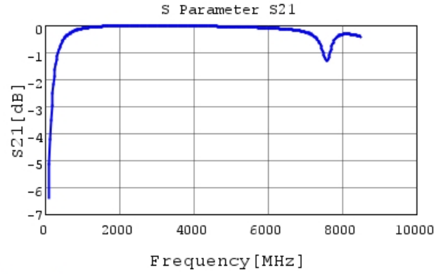
GJM1555C1H8R7WB01 S21 DCOV, 25degC
