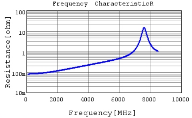
GJM1555C1H8R7WB01 R DC0V, 25degC
