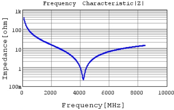
GJM1555C1H4R2WB01 |Z| DC0V, 25degC
