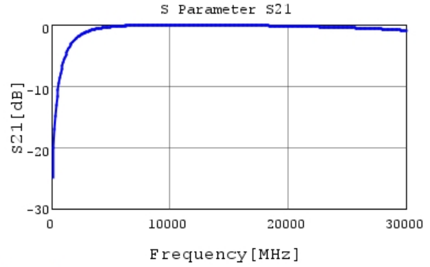
GJM0335C1ER90WB01 S21 DCOV, 25degC
