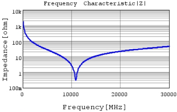
GJM0335C1ER90WB01 |Z| DCOV, 25degC
