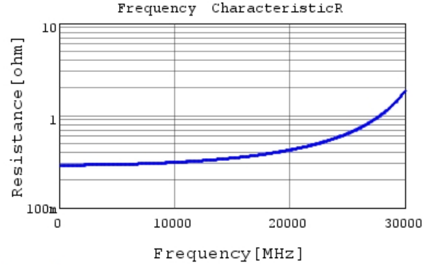
GJM0335C1ER90WB01 R DCOV, 25degC
