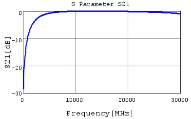
GJM0335C1ER60WB01 S21 DCOV, 25degC
