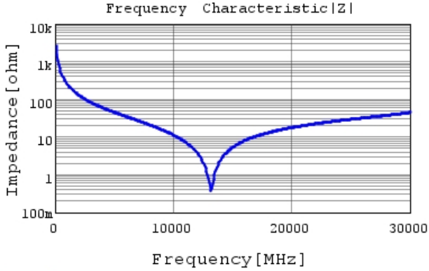
GJM0335C1ER60WB01 |Z| DCOV, 25degC
