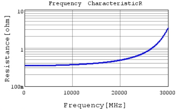
GJM0335C1ER60WB01 R DCOV, 25degC
