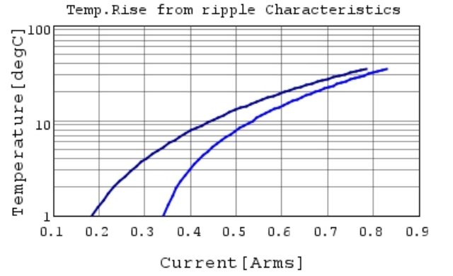
GJM0335C1H1R5WB01 Temp.rise — 3GHz — 4
