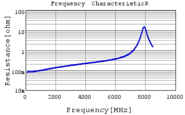
GJM1555C1H7R9WB01 R DC0V, 25degC
