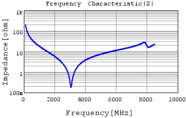
GJM1555C1H7R9WB01 |Z| DC0V, 25degC
