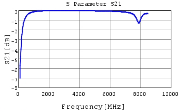
GJM1555C1H7R9WB01 S21 DCOV, 25degC
