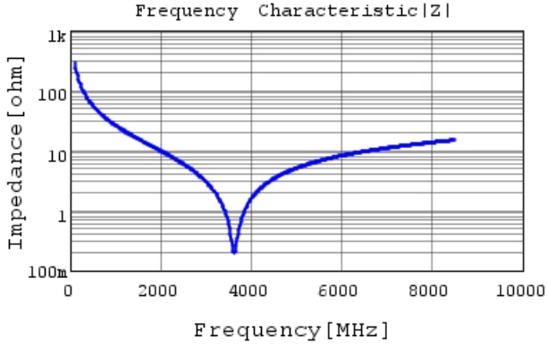
GJM1555C1H5R6DB01 |Z| DC0V, 25degC
