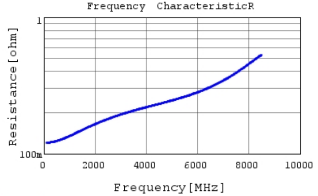
GJM1555C1H4R1WB01 R DCOV, 25degC
