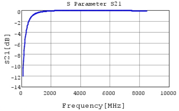
GJM1555C1H4R1WB01 S21 DCOV, 25degC
