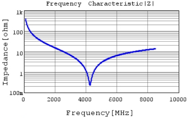
GJM1555C1H4R1WB01 |Z| DCOV, 25degC
