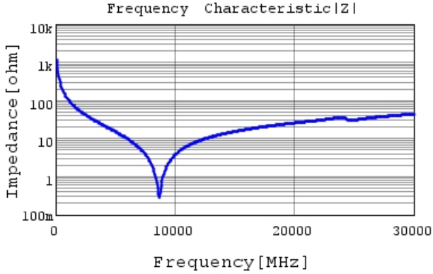
GJM0335C1H1R4WB01 |Z| DCOV, 25degC
