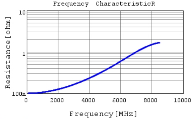
GJM1555C1H6R0WB01 R DCOV, 25degC
