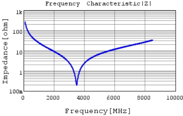
GJM1555C1H6R0WB01 |Z| DCOV, 25degC
