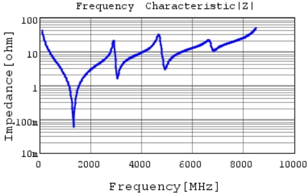
GQM1875C2E390JB12 |Z| DC0V, 25degC
