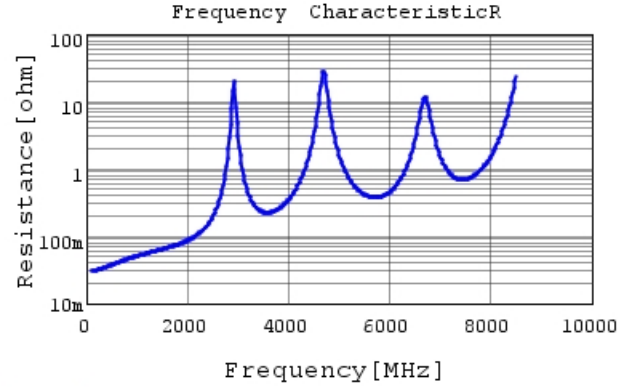
GQM1875C2E390JB12 R DC0V, 25degC
