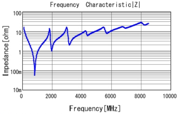
■ GQM1875C2E101GB12 |Z| DCOV, 25degC
