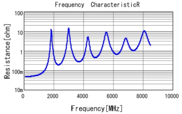
■ GQM1875C2E101GB12 R DCOV, 25degC
