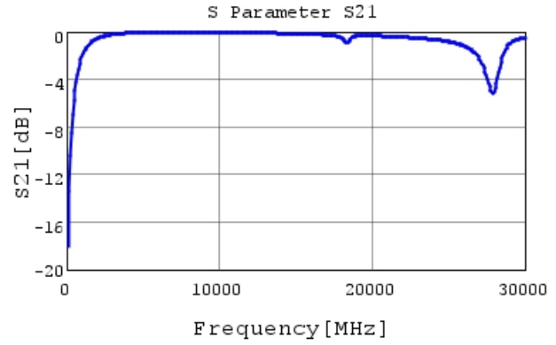
GJM0335C1H2R0WB01 S21 DCOV, 25degC
