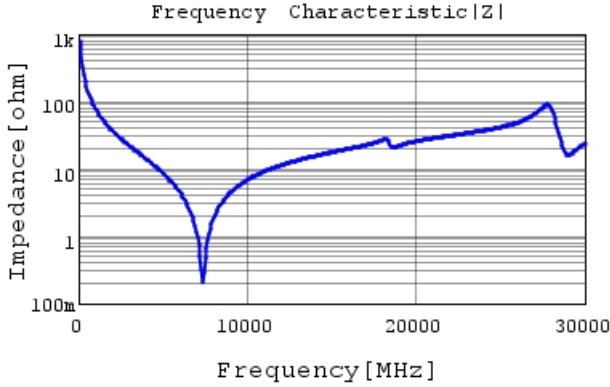
GJM0335C1H2R0WB01 |Z| DCOV, 25degC
