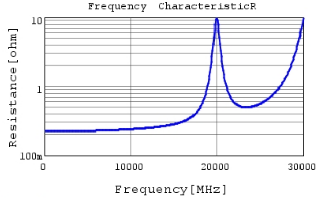
GJM0335C1H1R8WB01 R DCOV, 25degC
