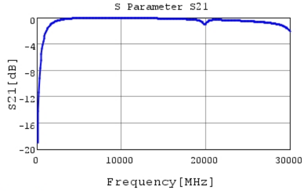
GJM0335C1H1R8WB01 S21 DCOV, 25degC
