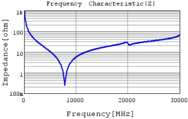
GJM0335C1H1R8WB01 |Z| DCOV, 25degC
