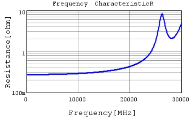
GJM0335C1H1R0WB01 R DCOV, 25degC
