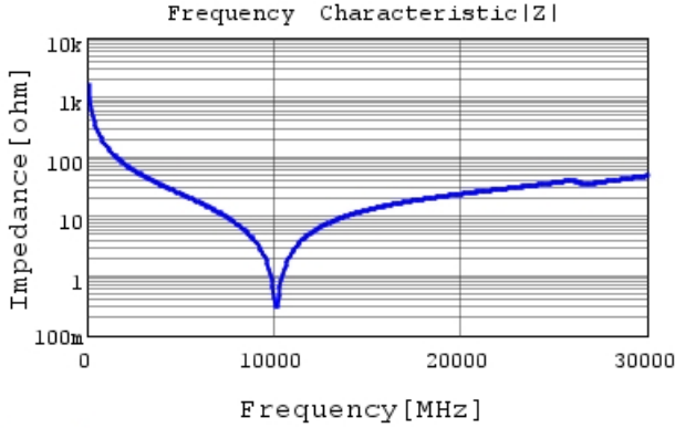
GJM0335C1H1R0WB01 |Z| DCOV, 25degC
