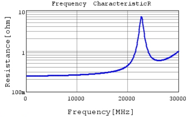
GJM0335C1H1R6WB01 R DCOV, 25degC
