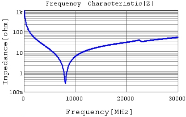
GJM0335C1H1R6WB01 |Z| DCOV, 25degC
