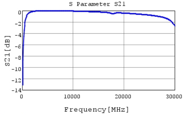
GJM0335C1E3R6WB01 S21 DCOV, 25degC
