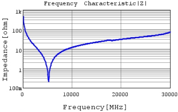
GJM0335C1E3R6WB01 |Z| DCOV, 25degC
