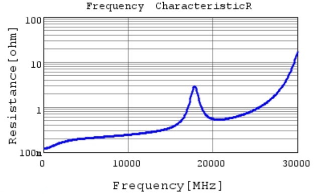
GJM0335C1E3R6WB01 R DCOV, 25degC
