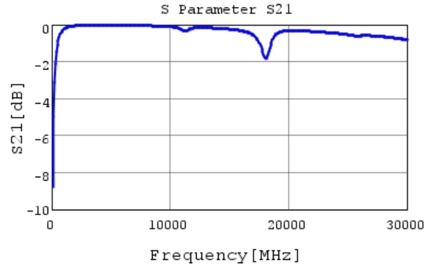
GJM0335C1E6R2WB01 S21 DCOV, 25degC
