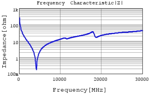
GJM0335C1E6R2WB01 |Z| DCOV, 25degC
