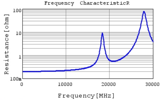
GJM0335C1E2R0BB01 R DCOV, 25degC
