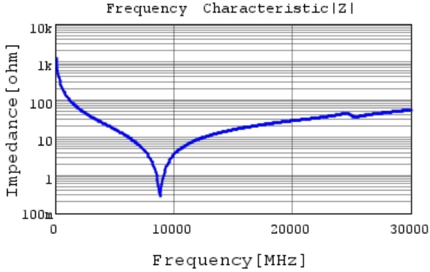
GJM0335C1H1R3WB01 |Z| DCOV, 25degC
