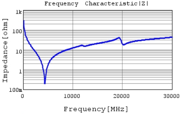
GJM0335C1E5R6WB01 |Z| DCOV, 25degC
