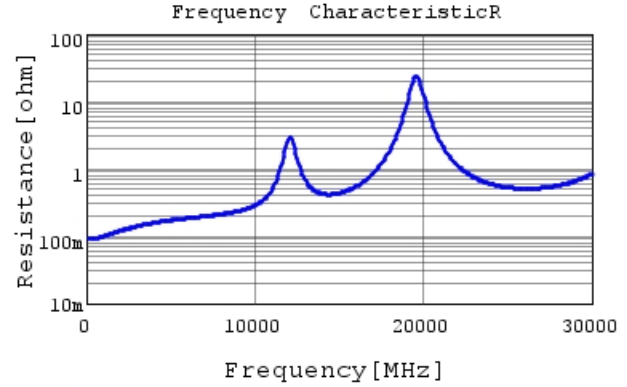
GJM0335C1E5R6WB01 R DCOV, 25degC
