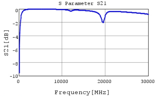
GJM0335C1E5R6WB01 S21 DCOV, 25degC
