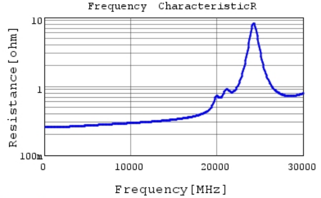
GJM0335C1E1R4WB01 R DCOV, 25degC
