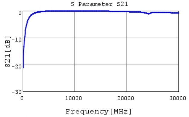
GJM0335C1E1R4WB01 S21 DCOV, 25degC
